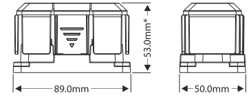
* Total height without cover is 43.5mm
