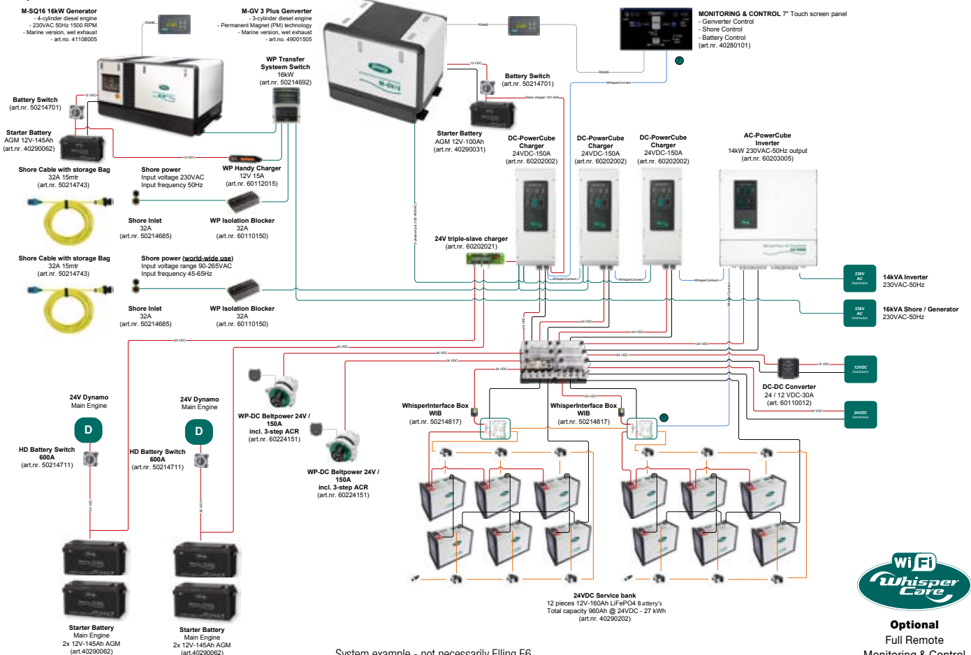
System example - not necessarily Elling E6
