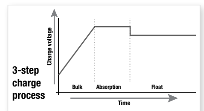
3 step charge curve with the supreme
