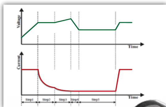
Graph illustrating multi step charge algorithm
