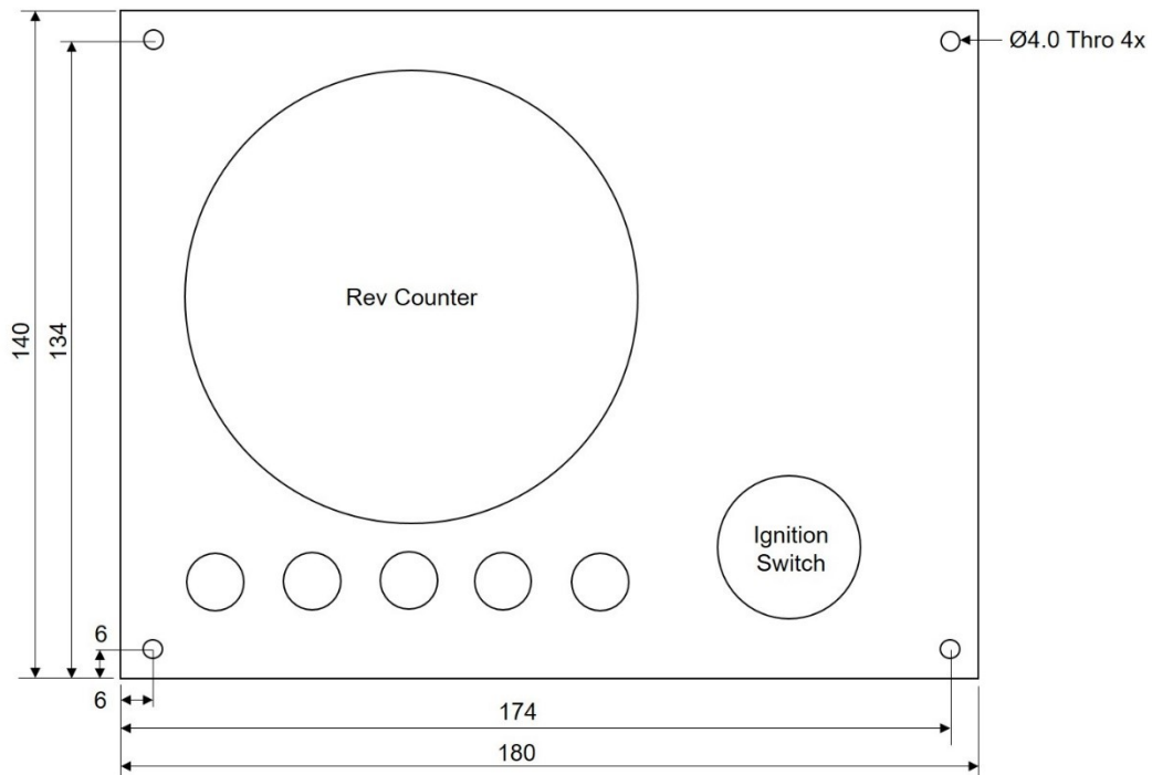
Figure 11: Standard Control Panel Dimensions
