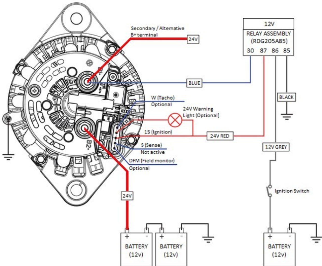
Figure 29: 24v 120A Alternator Wiring
