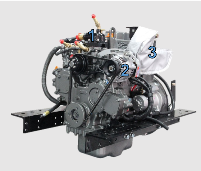
Figure 2: Shire 30 Left Side (Viewed from front)
