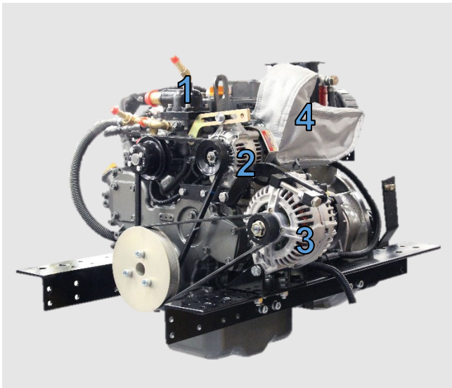
Figure 4: Shire 35 Left Side (Viewed from front)
