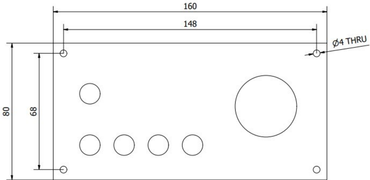
Figure 10: Basic Control Panel Dimensions
