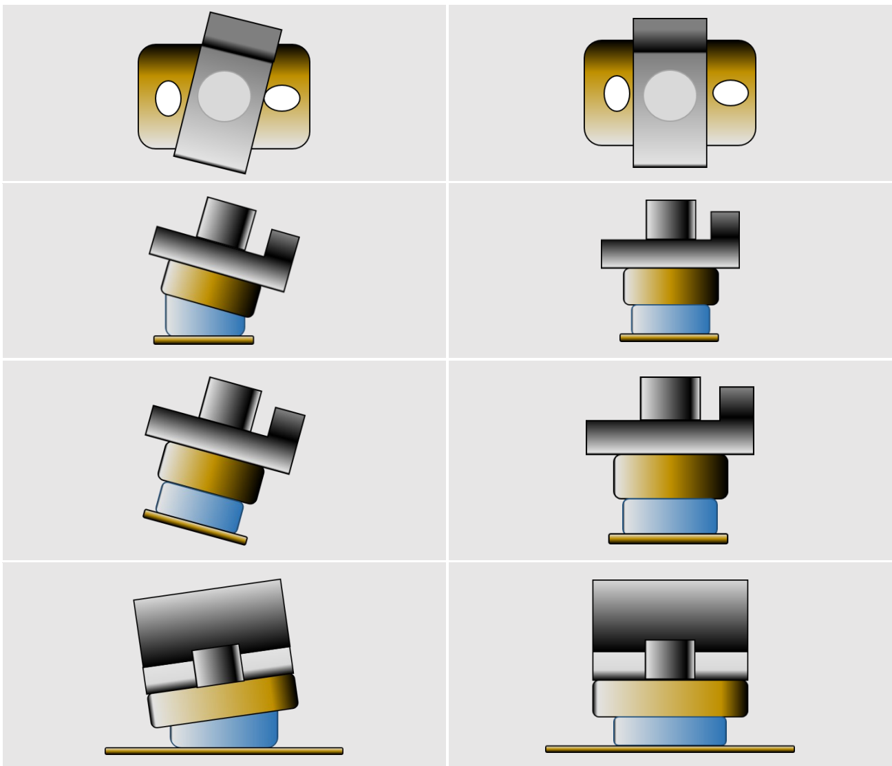
Figure 15: Correct Anti-Vibration Mount Installation
