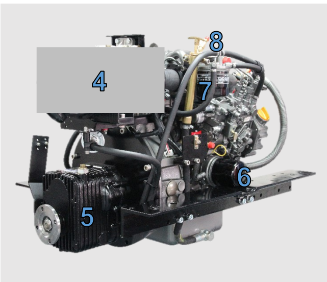
Figure 3: Shire 30 Right Side (Viewed from rear)
