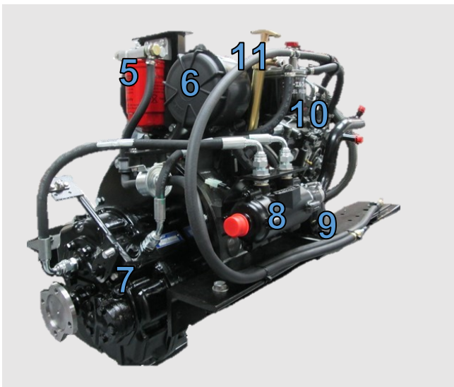
Figure 5: Shire 35 Right Side (Viewed from rear)
