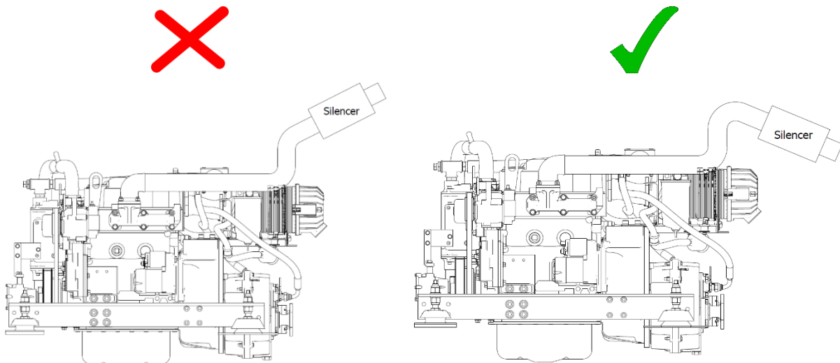
Figure 21: Correct Exhaust Installation
