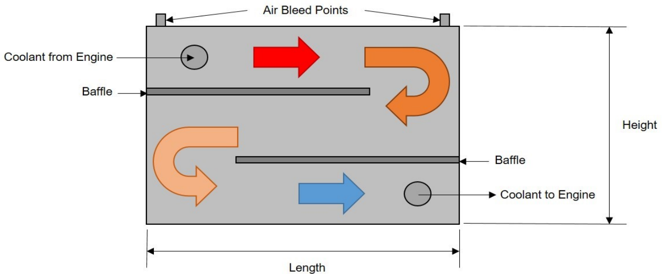
Figure 13: Skin Tank Flow Diagram
