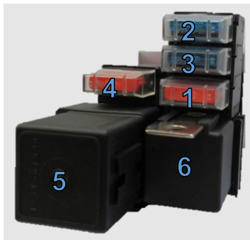
Figure 30: Fuses & Relays
