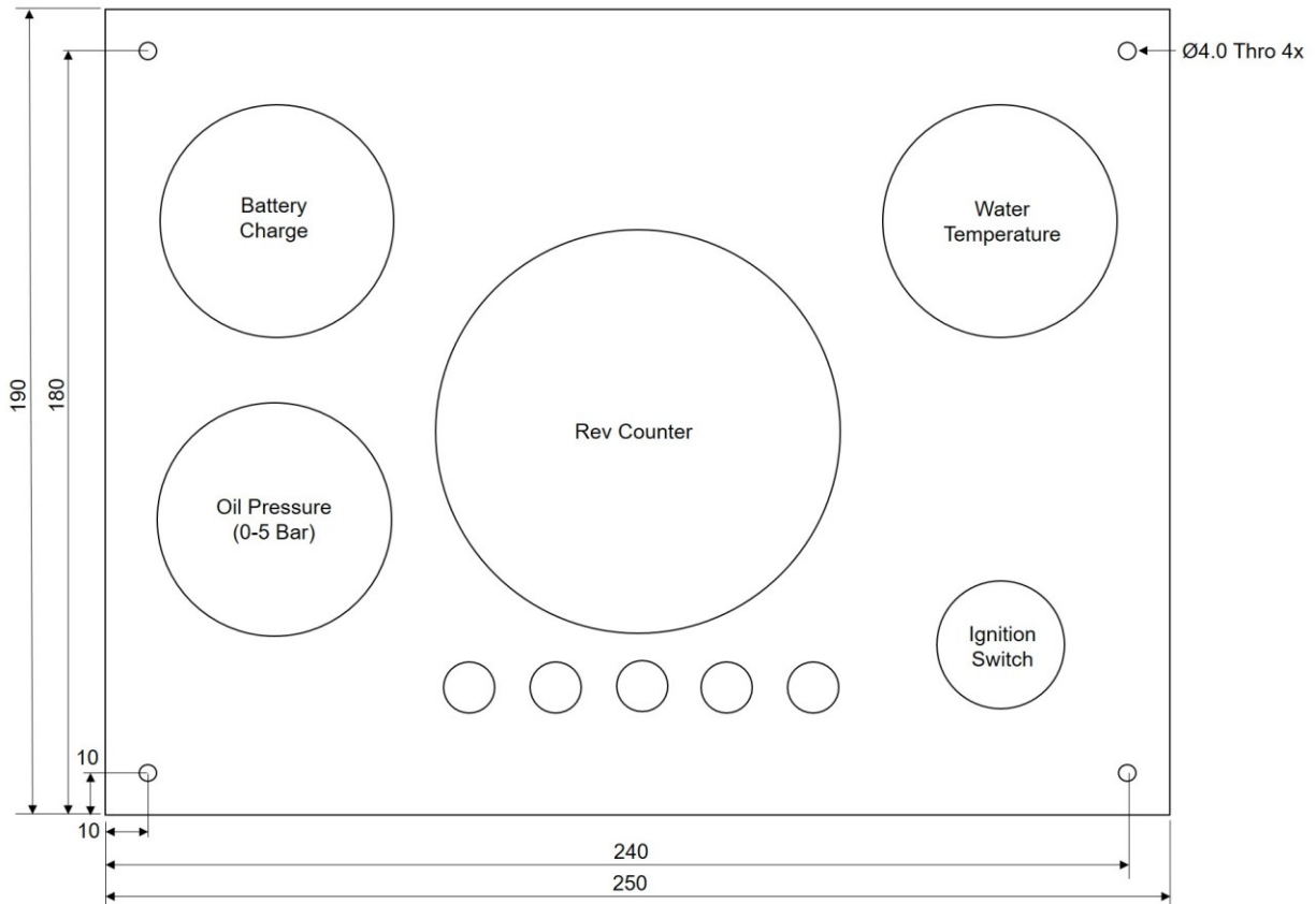
Figure 12: Deluxe Control Panel Dimensions
