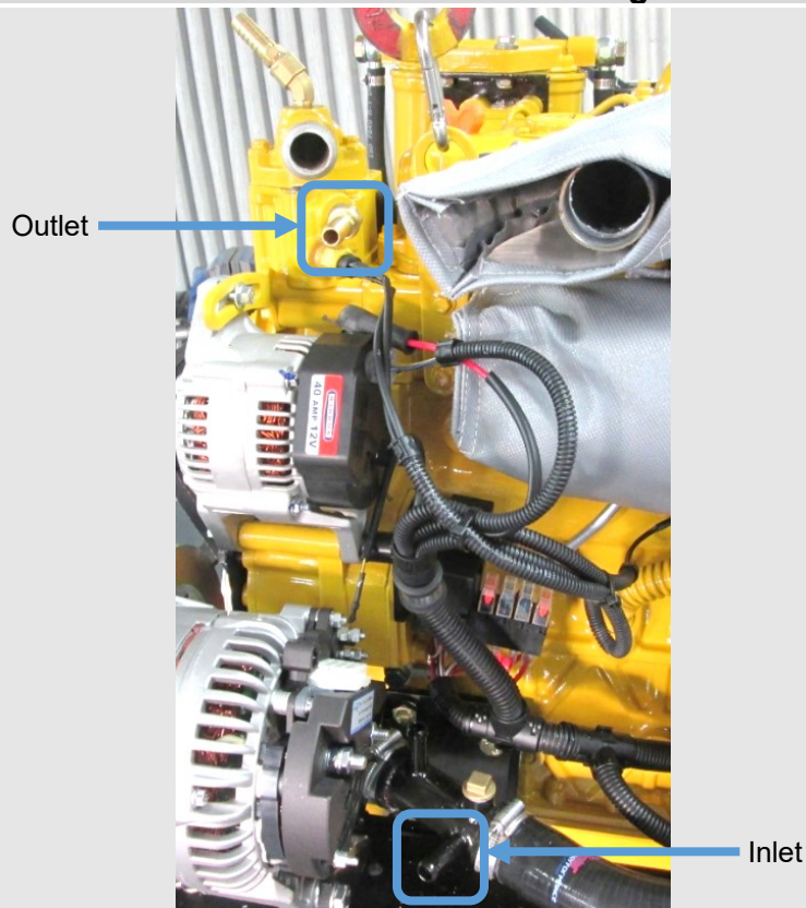
Figure 12: Calorifier Connections
