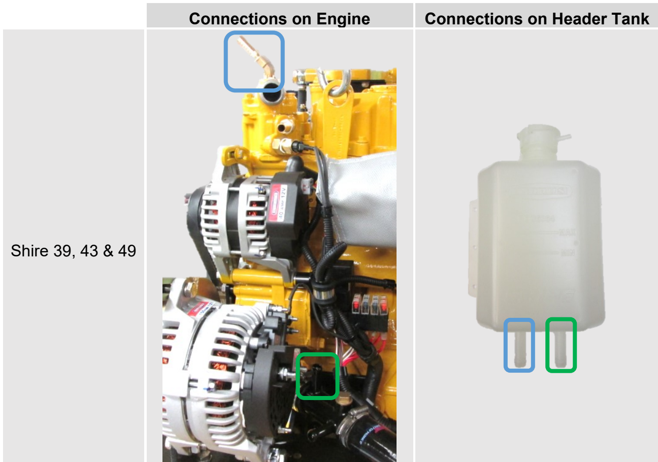
Figure 15: Header Tank Connections
