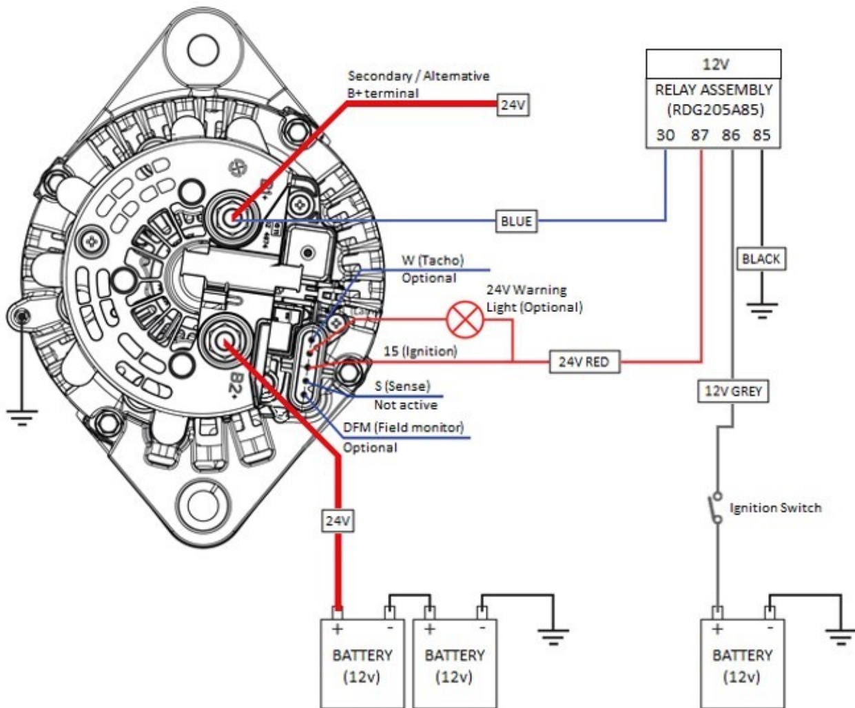
Figure 30: 24v 120A Alternator Wiring
