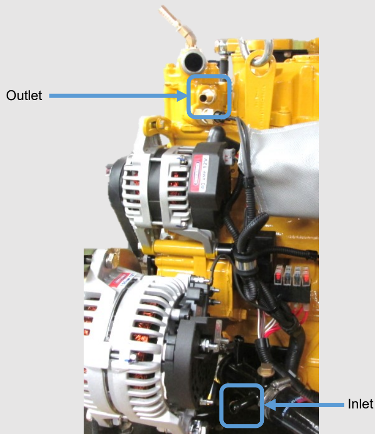
Figure 16: Calorifier Connections
