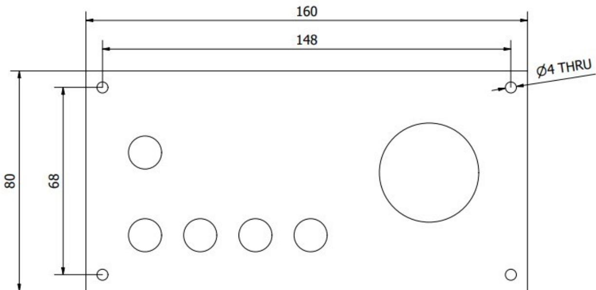
Figure 11: Basic Control Panel Dimensions
