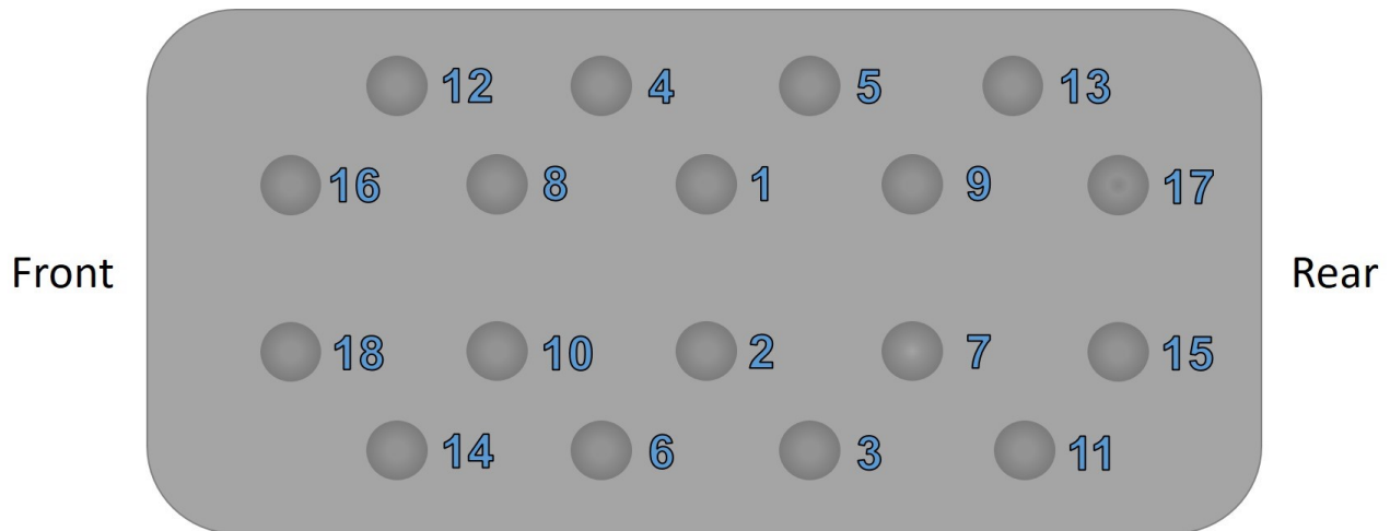
Figure 31: Cylinder Head Tightening Sequence
