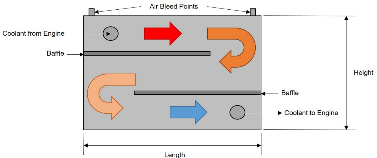
Figure 14: Skin Tank Flow Diagram
