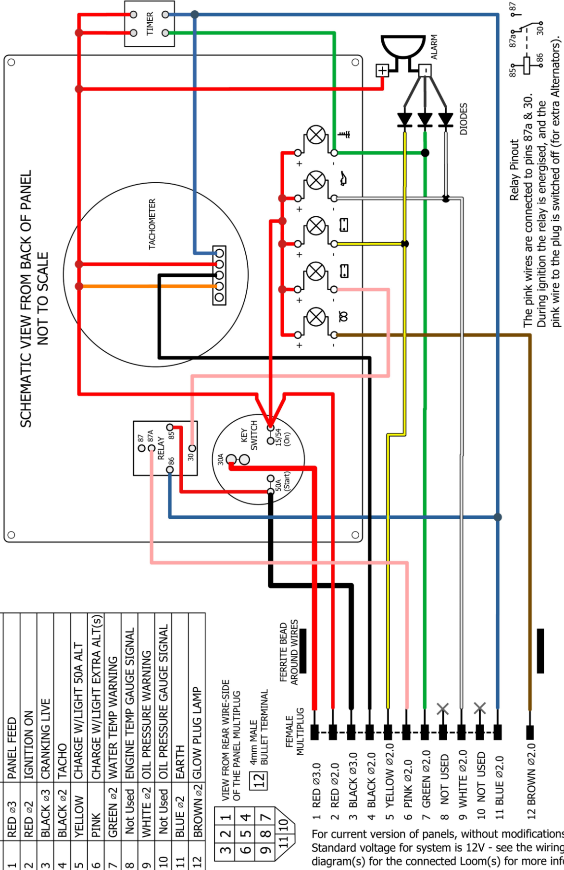
Figure 28: Standard Control Panel Wiring Diagram
