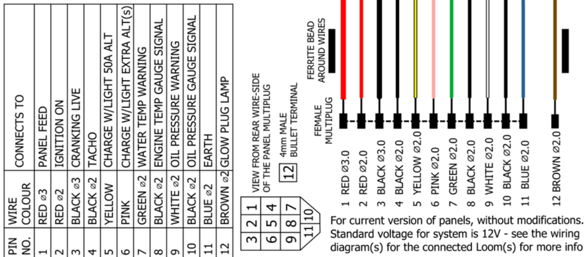
Figure 29: Deluxe Control Panel Wiring Diagram
