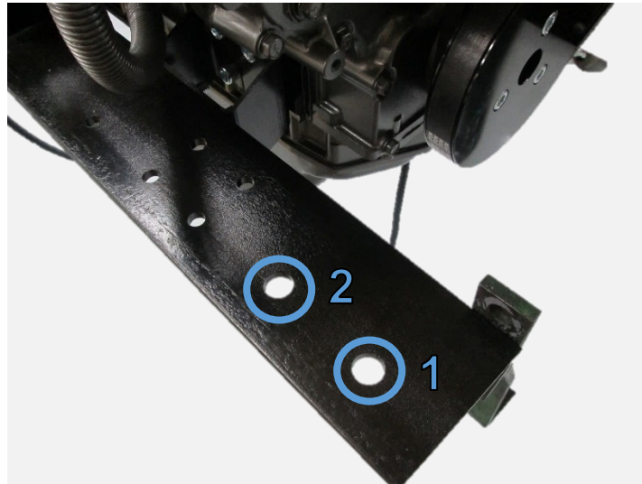
Figure 18: Correct Anti-Vibration Mount Installation
