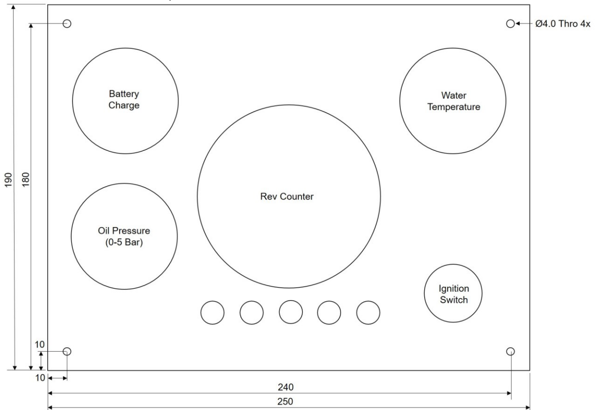
Figure 13: Deluxe Control Panel Dimensions
