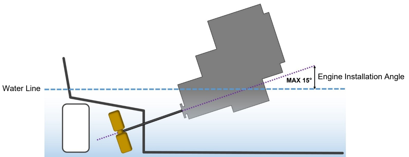
Figure 20: Maximum Engine Installation Angle
